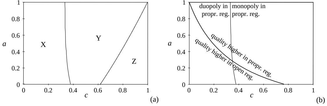
Figure 4: Comparison of equilibria under proprietary and open regime. (a): Market structure. Proprietary regime: duopoly in X, monopoly in Y, Z. Open regime: Duopoly in X, Y, monopoly in Z. (b): Product qualities. Border curve given by a_q(c) , equation (27).
